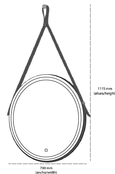
203300-N ROUND LEATHER LED Acabado: negro mate. Finish: matte black. Ø 70 cm.
