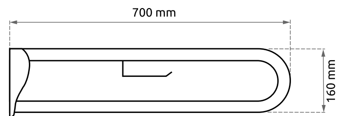
ASIDERO ABATIBLE 180° 180° FOLDING GRAB RAIL
